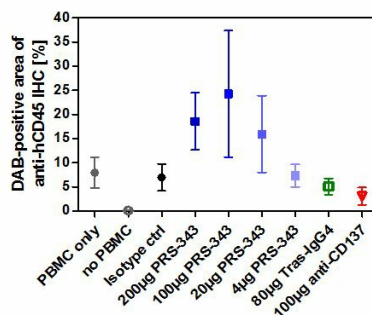
Figure 5 Cinrebafulp alfa activity in mice engrafted with HER2-positive SK-OV-3 cell line and human PBMC. (A) Median of tumor growth. (B) Frequency of CD45+ cells determined by immunohistochemistry of tumors after study end.
