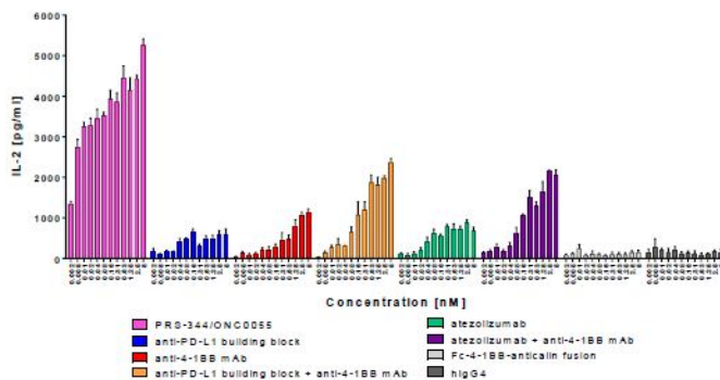
Figure 1 The combination of anti-PD-L1 benchmark and anti-4-1BB benchmark demonstrates the strong synergistic effect of T cell co-stimulation and checkpoint blockade in T cell activation. With PRS-344, this synergistic effect is massively increased.
